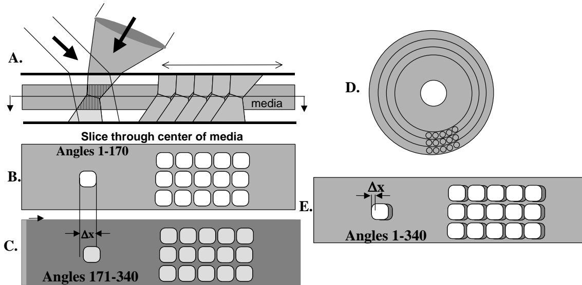
Figure 2: Illustration of Short-Stacking. See text for explanation
