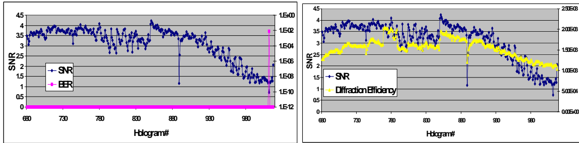
Figure 4: Data from our 350 Gbit/in 2 experimental demonstration. This data is taken from the last book containing two short-stacks of 170 holograms each. Left: Bit Error Rate (BER) and SNR. Right: SNR and Diffraction Efficiency.
