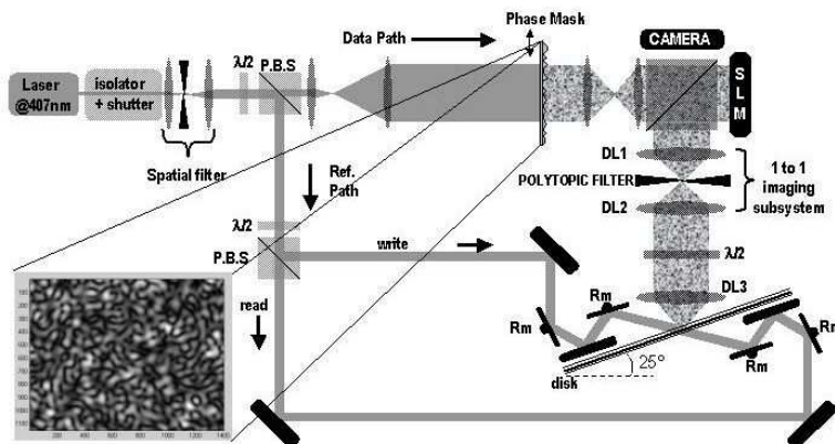
Figure 1: System layout of Polytopic Phase Conjugate Geometry with a moving phase mask imaged onto the SLM
